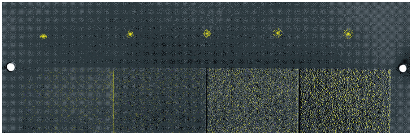
Test Block Type 2 according to DIN EN ISO 3452-3
